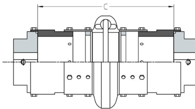
DOUBLE EXTENSION
